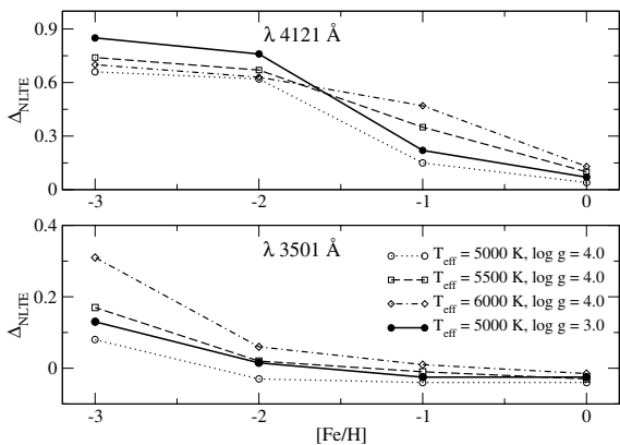
Figure 4. NLTE abundance corrections \Delta_{\text{NLTE}} calculated for the lines of Co I (4121 Å, top) and Co II (3501 Å, bottom). Calculations are performed for 16 models with T_{\text{eff}} = 5000, 5500, 6000 K; \log g = 3, 4 ; [\text{Fe}/\text{H}] = 0, -1, -2, -3 .
