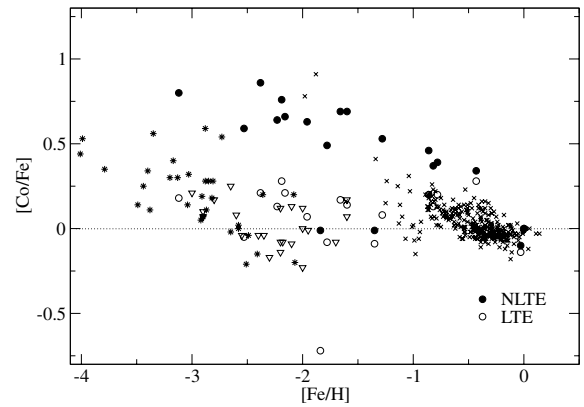
Figure 6. [\text{Co}/\text{Fe}] versus [\text{Fe}/\text{H}] in metal-poor stars. The Co abundances are derived from Co I lines under NLTE (filled circles) and LTE (open circles). Iron abundances are determined from Fe II lines in LTE. The sources of other LTE [\text{Co}/\text{Fe}] data are Johnson (2002) (open triangles), Reddy et al. (2003, 2006) (crosses) and McWilliam et al. (1995) (stars).
