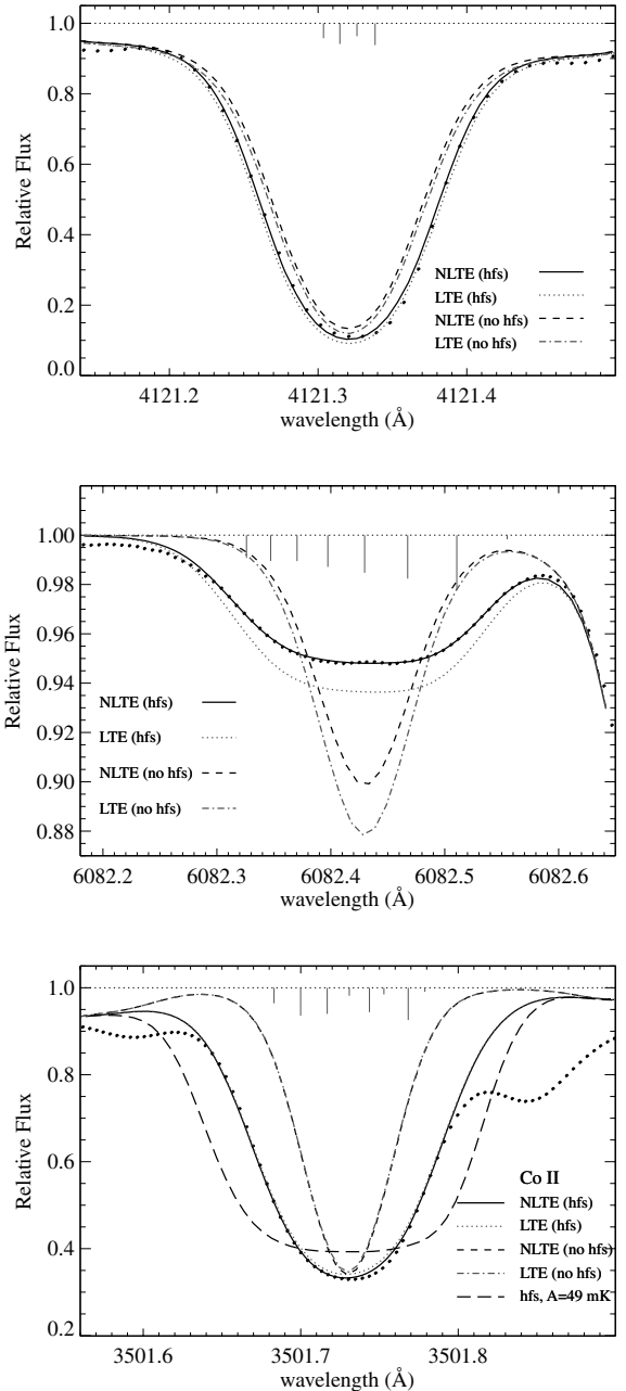
Figure 3. The lines of Co I (4121, 6082 Å) and Co II (3501 Å) in the solar flux spectrum (filled circles). Synthetic NLTE and LTE profiles with and without HFS are labelled correspondingly. Wavelength positions and relative line strengths of the HFS components are indicated. Note that the relative HFS component intensities are not on the same scale in figures. The long-dashed trace on the bottom figure indicates the NLTE profile computed with A = 49 mK for the lower level a^5P_3 (our reference value is A = 40 mK).
