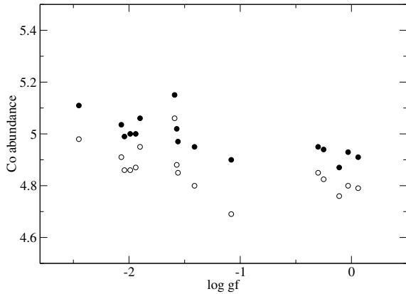
Figure 5. Abundances of the 17 solar Co I lines. NLTE and LTE abundances are marked with filled and open circles, respectively.
