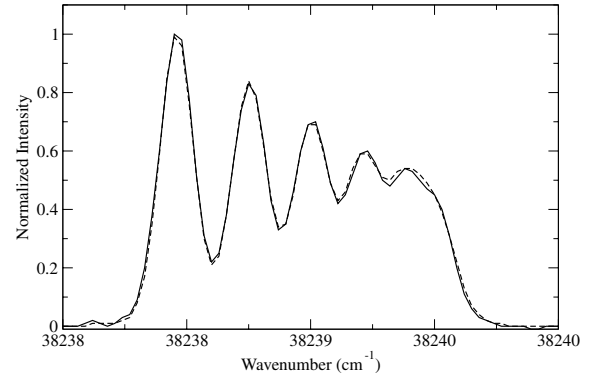
Figure 1. An example of an observed (heavier trace in plot) and fitted (dashed trace) line profile, for a Co II transition recorded by FTS: (38\,238.965 \text{ cm}^{-1})\,2614.3530 \text{ \AA} transition, 3d^7 ({}^4P)4s a^5P_3 - 3d^7 ({}^4P)4s z^5D_2^0 .
