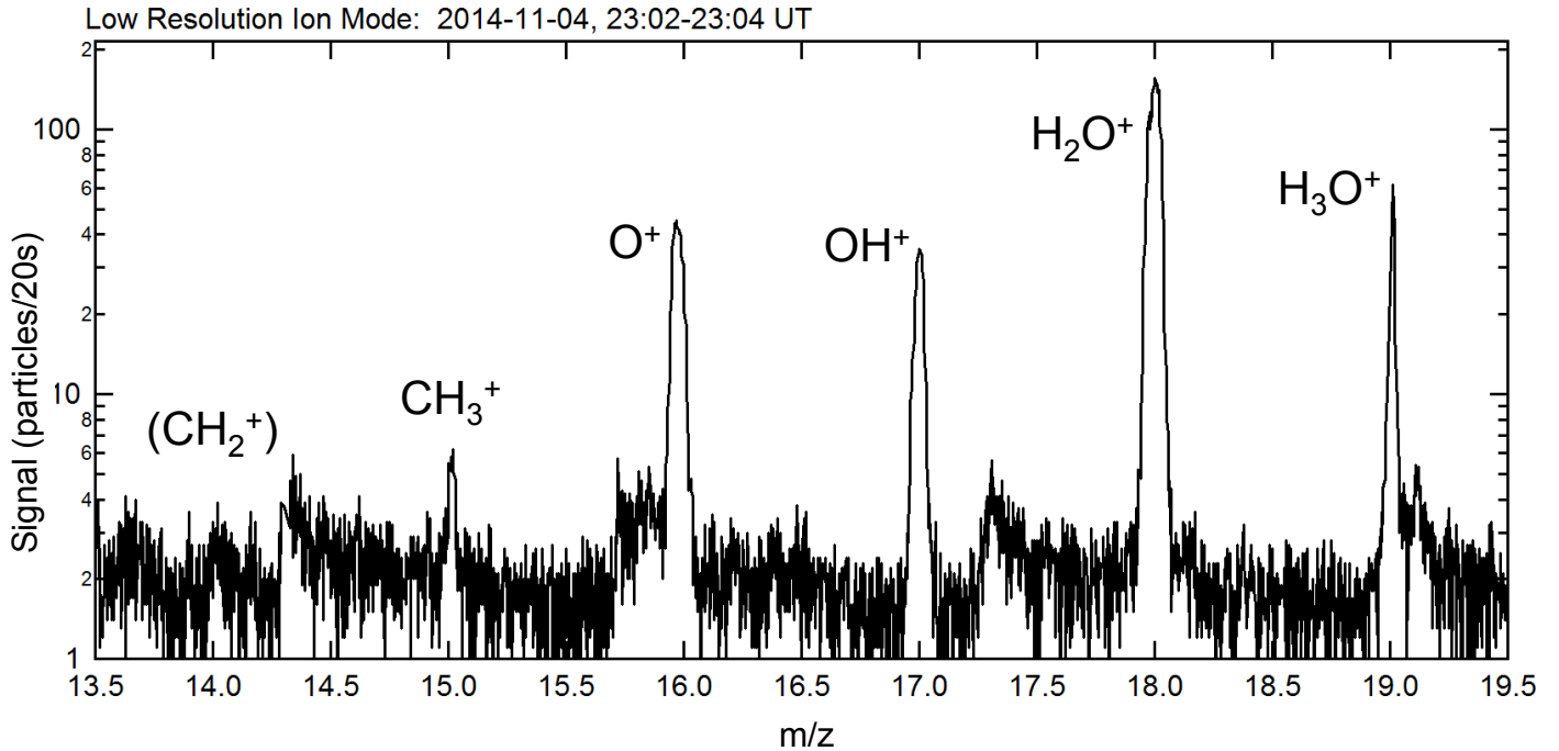
Fig. 5. Low-resolution ion spectrum from mass 13.5 to 19.5 u/e. There may be a peak at mass 14 (probably \text{CH}_2^+ ) and there are certainly peaks at mass 15 through mass 19 (primarily water group ions, with \text{H}_3\text{O}^+ at mass 19, and \text{O}^+ , \text{CH}_3^+ , at mass 16 and 15, respectively). Apparent peaks at masses 13.6, 14.4, and 17.4 are not real. They are the result of a combination of mass spectra with a gradient in the offset across the DFMS detector.
