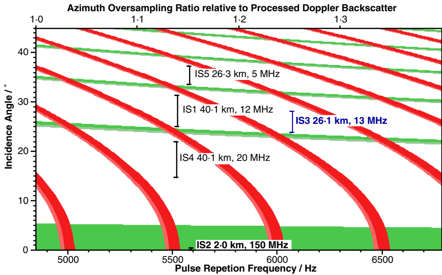
Fig. 3 Swath selection diagram. Image swaths must avoid both the red (antenna transmitting) and green (nadir echos received) areas
