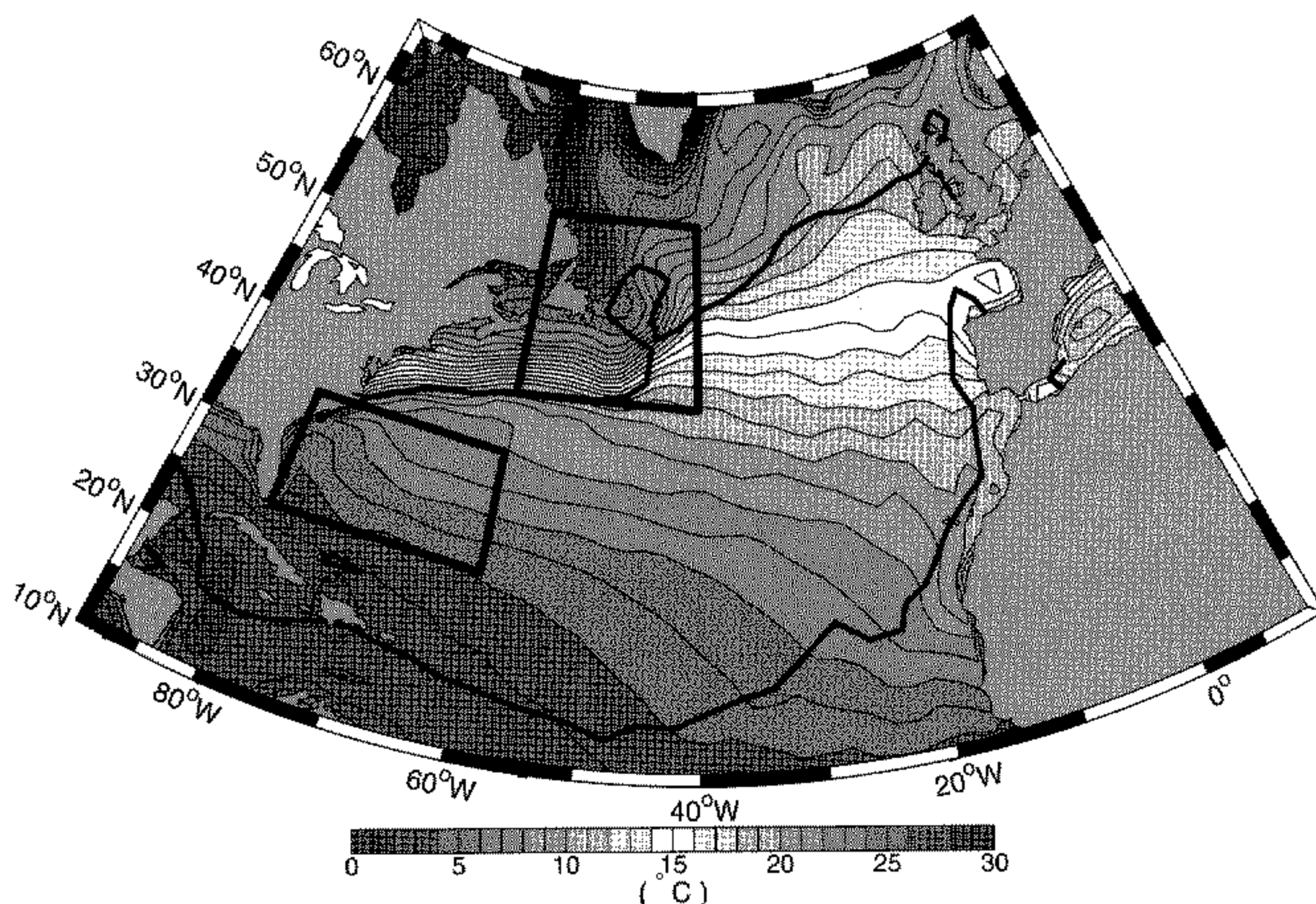
Figure 1. Annual mean sea surface temperature (SST) (grey shading) and position of the zero wind-stress-curl line (thick black lines) from the NCEP climatology (1961–90). The two black boxes indicate the regions used to construct the dipole SST index \Delta T = T_N - T_S , where T_N is the temperature in the northern box and T_S the temperature in the southern box.
