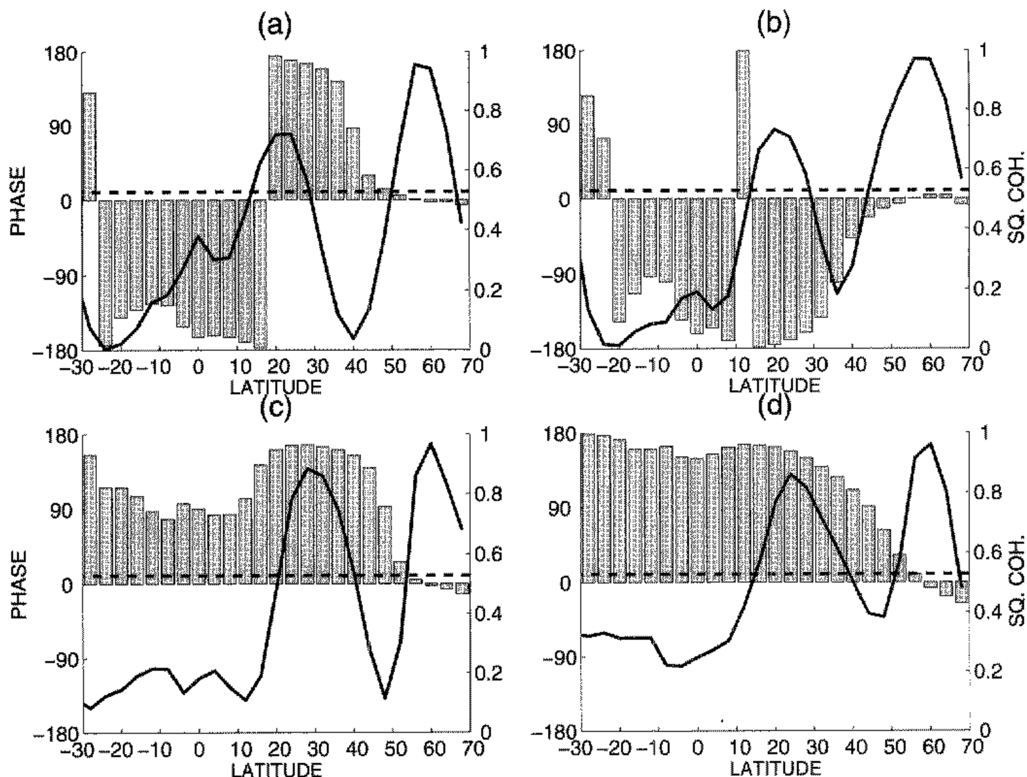
Figure 10. Same as Fig. 9 but for the Greenland-Iceland Low instead of \Delta T .
