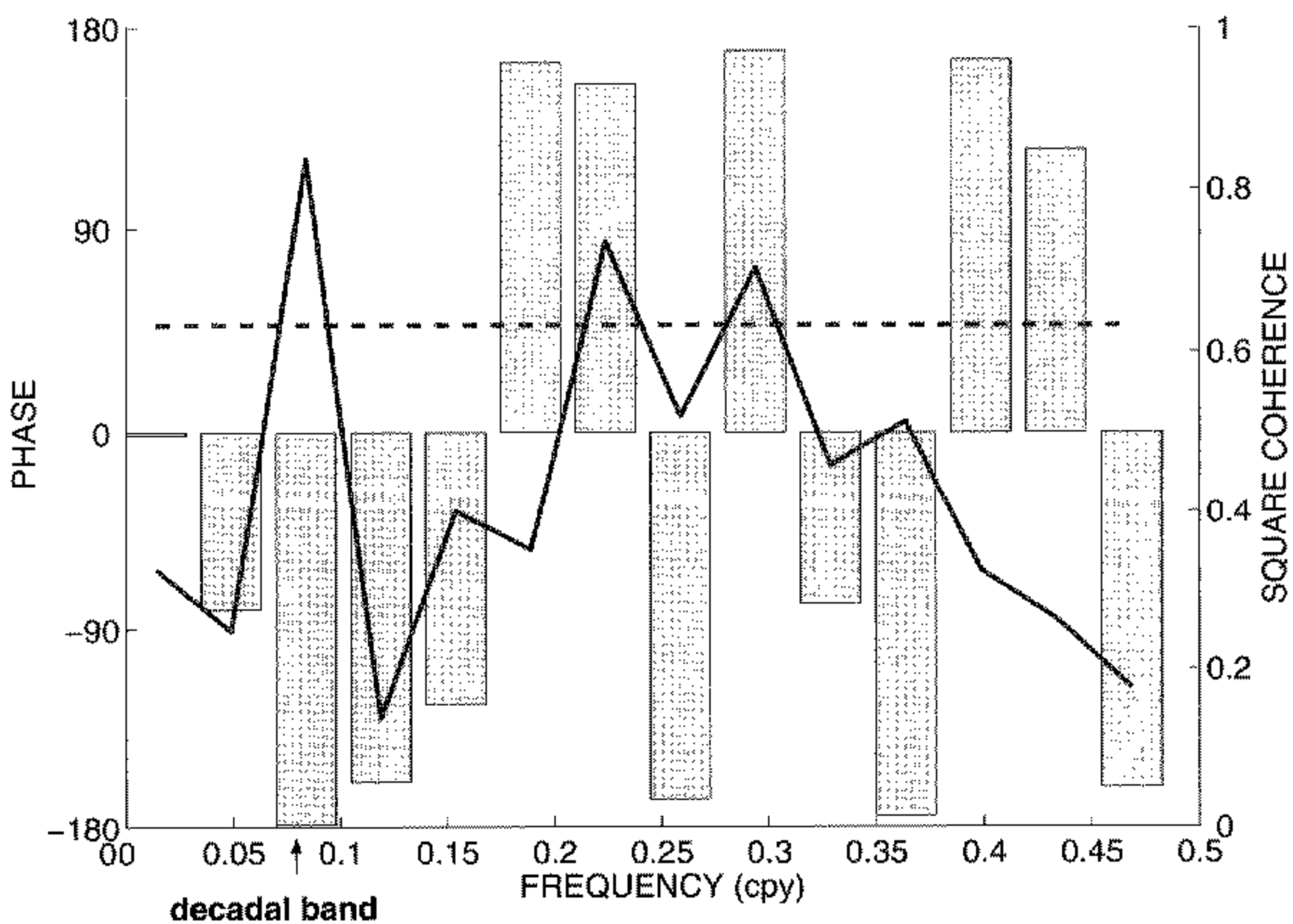
Figure 5. Phase spectrum (bars, in degrees as indicated on the left y-axis) and squared coherence (thick curve, right y-axis) between T_N and T_S (see text) as a function of frequency (in cycles per year). The width of the Daniell window M has been set to 5, and the corresponding level of significance for the squared coherence at the 95% level is indicated as the dashed horizontal line (see section 2).
