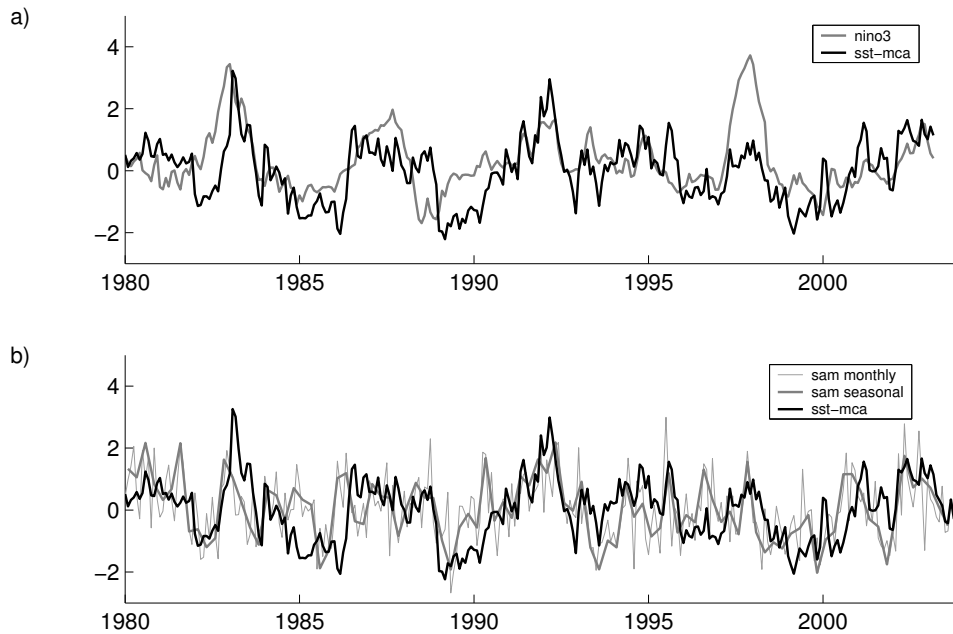
FIG. 7. Time series of SST-mca, black line, in both panels. a) Niño3 (gray line) and b) SAM index (thin gray, monthly data, thick gray, seasonal averages). Each index is normalized.
