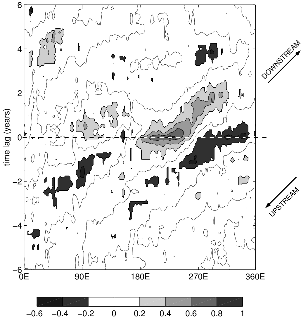
FIG. 4. Lagged correlation of observed SST with the first SST-mca mode (from Figure 3). At zero lag, following the horizontal dashed line, the pattern of Figure 3a is retrieved. Lighter shades of gray indicate positive correlations and darker shades, negative correlations; only values that are significant at the 95% level are shown. The location of the maximum correlation ( \sim 210\text{E} at zero lag) is displaced to the right as lag increases, indicating eastward propagation of the signal. The speed of propagation is estimated from the Figure to be 8\text{ cm/s} , which coincides with the mean advection velocity of the ACC. If they persisted, anomalies would encircle the globe in approximately 10 years.
