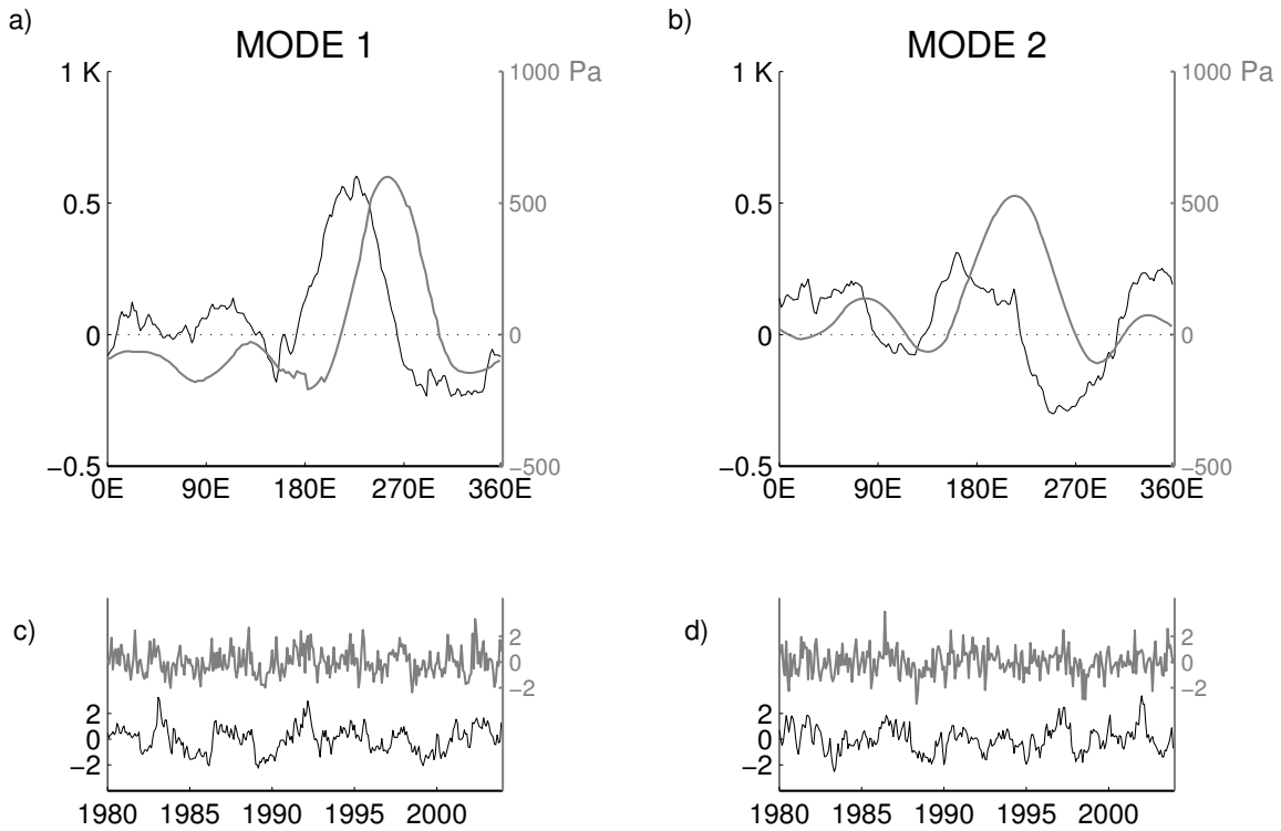
FIG. 3. First and second modes of variability of SST (black) and SLP (gray) showing the maximum covariance along the ACC. The spatial patterns for mode 1 and 2 are presented in a) and b) respectively. Mode 2 is upstream of mode 1 and has weaker amplitude. The amplitude shown corresponds to a typical change in SST (in K ) or SLP (in Pa ) for a 1 standard deviation of the associated time series. The normalized time series associated with the spatial patterns are presented in c) and d).
