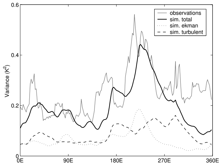
FIG. 6. Variance of SST as a function of longitude (along the path of the SST). Gray line: observations; dotted line: simulated from Ekman heat fluxes; dashed line: simulated from surface heat fluxes; black solid line: simulated from Ekman + surface heat fluxes.
