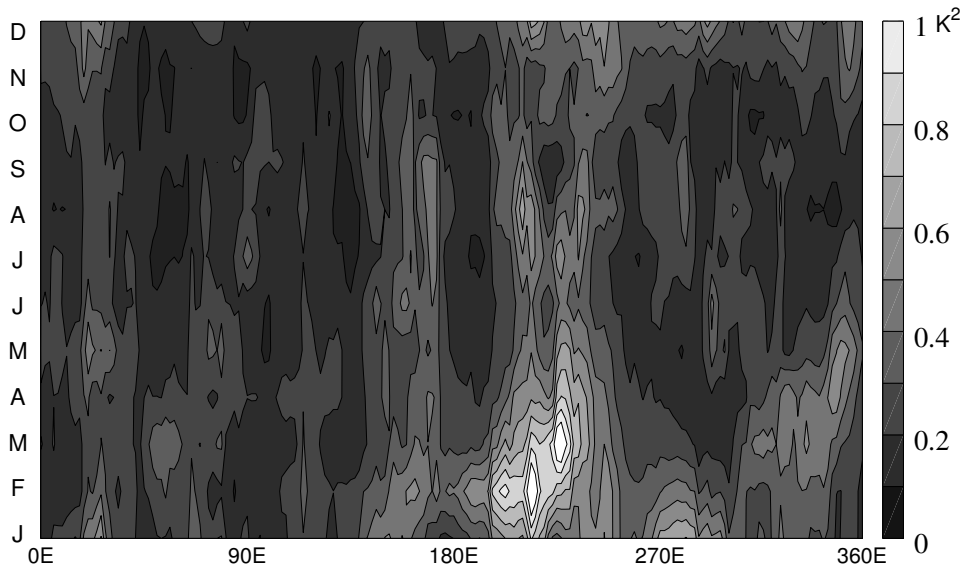
FIG. 2. Variance of SST anomalies along the ACC (x-axis is longitude), as a function of calendar month. The variability is greatest in the Pacific sector (200E to 300E); it is enhanced during the Austral summer when the mixed layer is shallowest.
