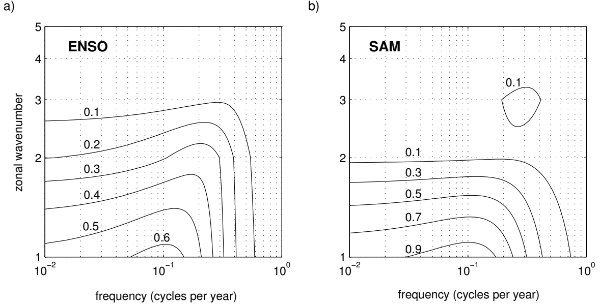
FIG. 11. Wavenumber-frequency spectrum for SST, as predicted from Equation 4, assuming a white-noise forcing with the spatial pattern of a) the heat fluxes regressed on ENSO, as shown in Figure 9e; and b) the heat fluxes regressed on SAM, as shown in Figure 9f. Both spectra are normalized by the peak value of the SST spectrum in b). The ocean response is expected to be at low wavenumbers, with a dominant period of 10 years. Note that the spectrum is continuous in \omega but discrete in k . The spectra were calculated with \lambda = \alpha \simeq (9 \text{ months})^{-1} .
