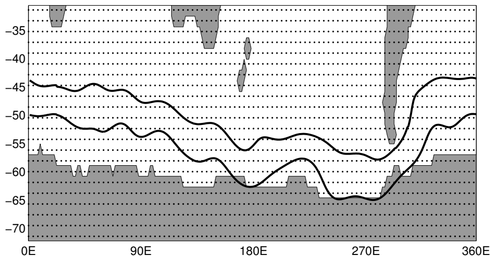
FIG. 1. Two geostrophic streamlines encircling the globe, delimiting the region of the ACC, plotted over the data grid points (from NCEP-NCAR Reanalysis); for clarity only half the points are shown in the zonal direction. Shaded areas represent land masses and sea ice.
