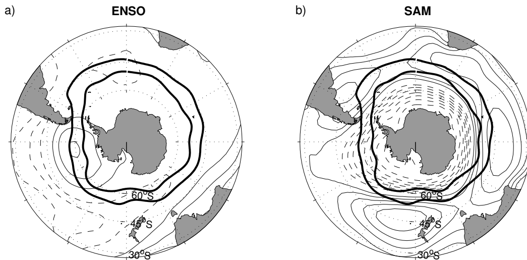
FIG. 8. Correlation of SLP with a) Niño3 index and b) SAM index; solid (dashed) contours indicate positive (negative) correlations. The contour interval is 0.1; the zero contour is not drawn. Thick black lines show the mean position of the ACC as defined in Section 2. In the ACC band, both signal exhibit a strong pressure anomaly in the South-East Pacific.
