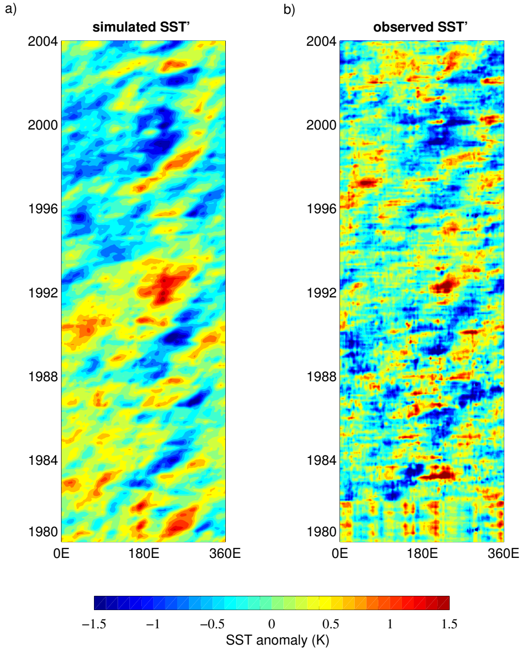
FIG. 5. Time-longitude diagrams of a) the SST simulated from the heat fluxes, estimated from the Reanalysis and introduced in Equation 4; b) observed SST from the Reanalysis. The simulated field captures the propagation and timing of the observations.
