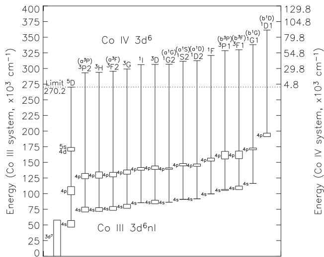
Figure 5. Term diagram of the singly excited system of Co III with the subconfigurations, 3d^6(M)Lnl , based on the parent terms, M_L , of the 3d^6 ground configuration of Co IV, showing the experimentally established energy levels.
