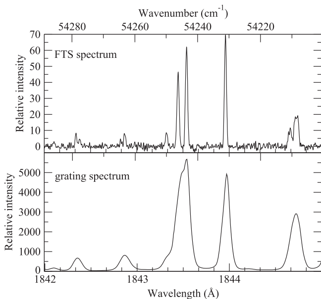
Figure 3. A comparison between the FTS (top) and grating (bottom) spectra for Co III in the wavenumber region 54,200\text{ cm}^{-1} – 54,290\text{ cm}^{-1} ( 1845.0 – 1842.0\text{ Å} ).
