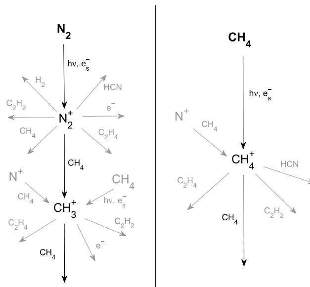
Figure 1. Chemical reactions considered for calculation of N_2^+ and CH_4^+ production rates. “ h\nu, e_s^- ” corresponds to ionization by solar photons and by impact with suprathermal electrons.
